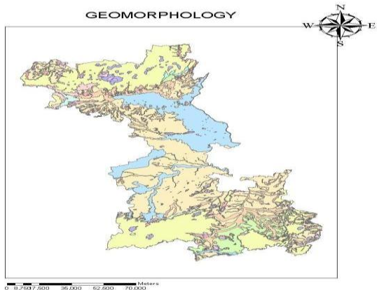
Figure.5.2 Geomorphology Map
